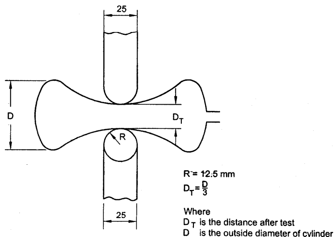
FIG. 4 CRUSHING TEST
