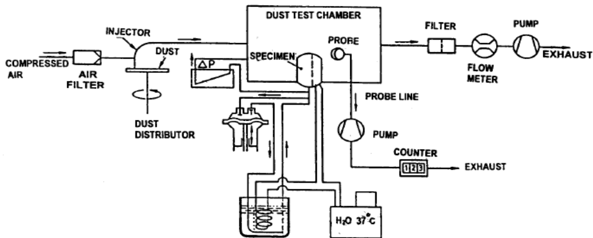
Figure 2 Typical Sinusoidal Dolomite Dust Test Equipment/Setup for Clogging Test
