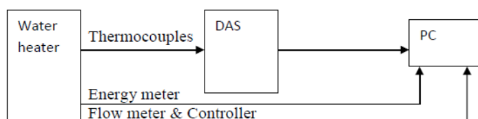
Schematic Diagram for one module when data for energy and flow is fed directly into PC
