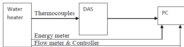
Schematic Diagram for one module when data for energy and flow is fed directly into PC
