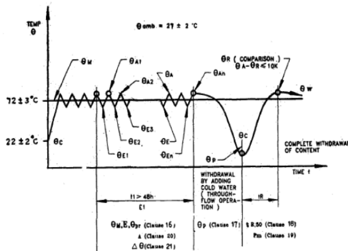
FIG. 4 MEASUREMENT FOR THERMAL STORAGE WATER HEATERS
